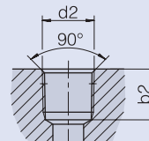
Threaded bore NPT ASME B 120.1 for tapered threads
