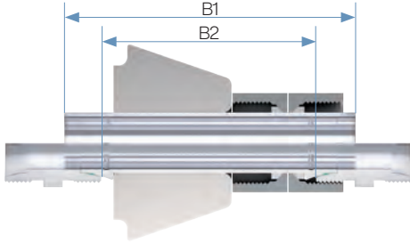
Minimum lengths for clamping in curved tubes ( R \geq 3 \times \text{tube OD} )
