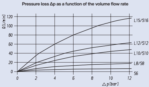
Flow resistance
