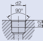
Threaded bore DIN 3852-1 and -2 form Z 1) (for tube connection stubs with tapered threads)
