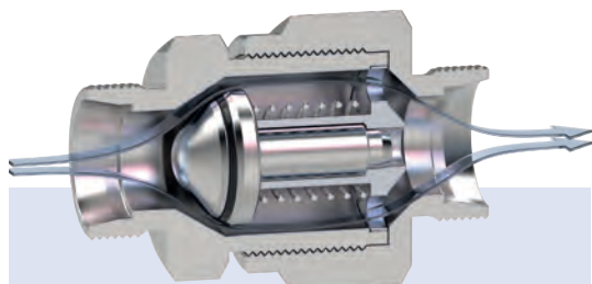
Flow-optimized geometry
